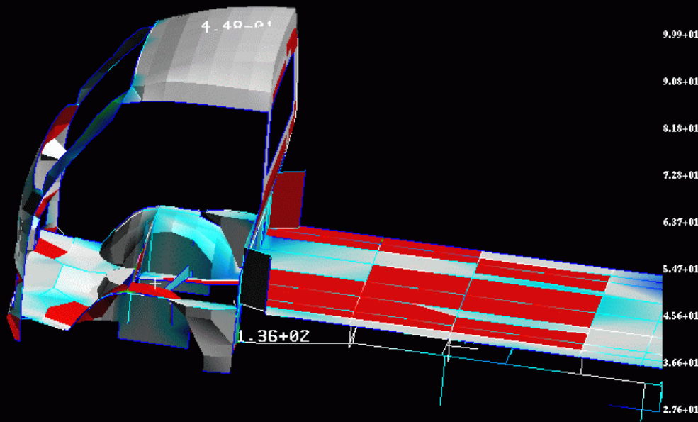
figure 1 bend case static strength analysis
