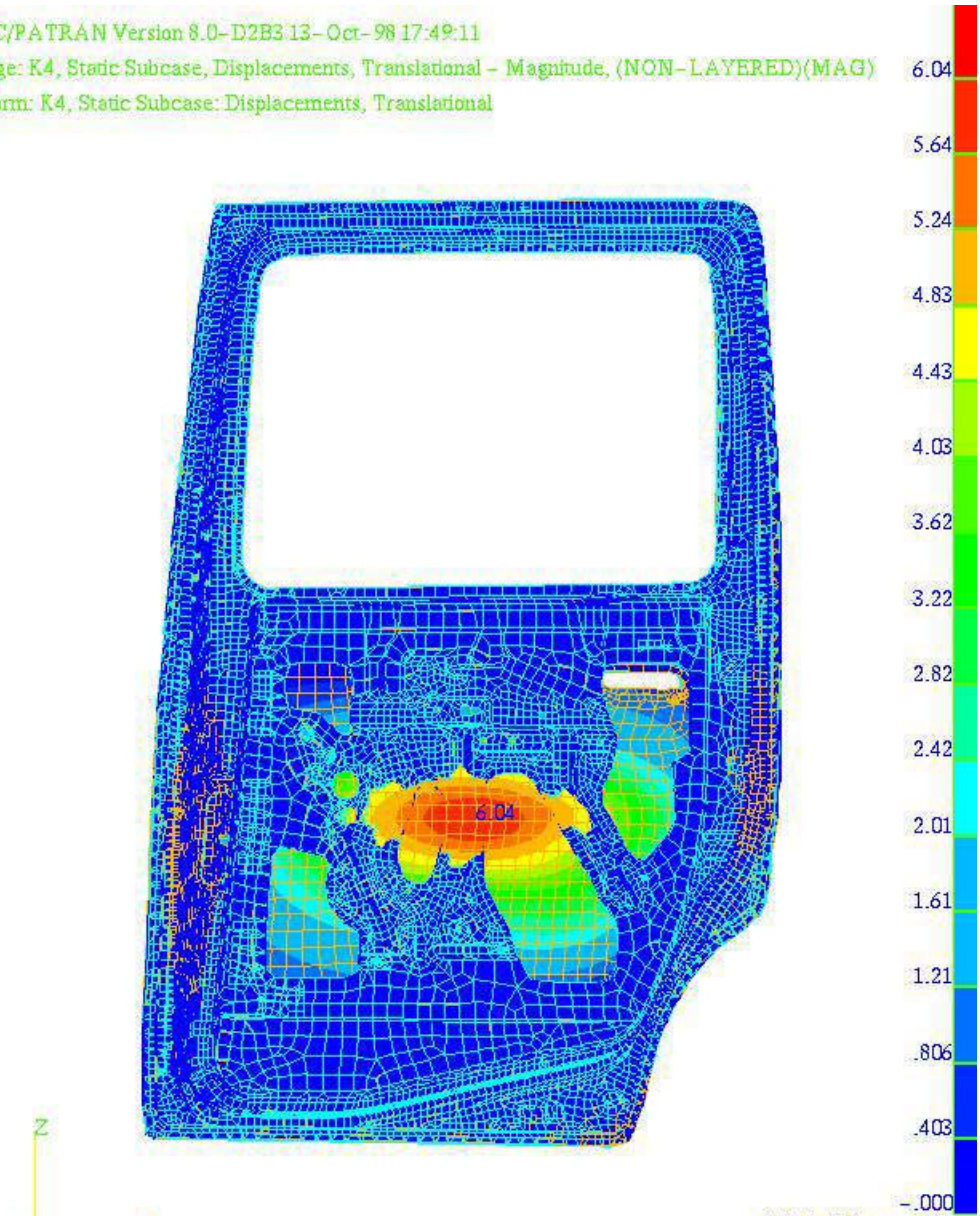
figure 9 door stiffness analysis
