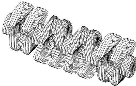
Figure 3. Crankshaft model
