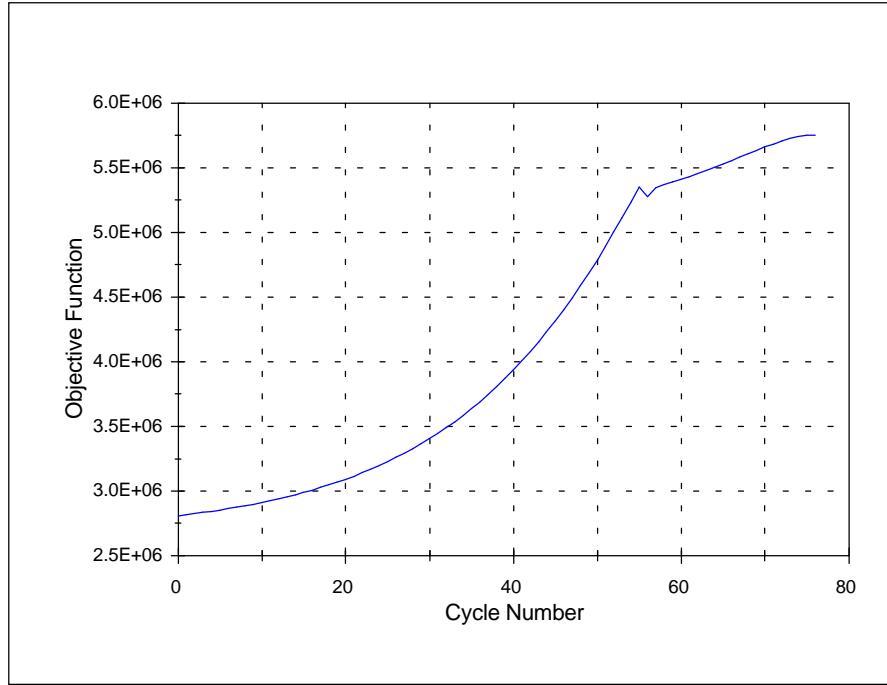
Figure 2. Stiffness history for 2x2 layout
