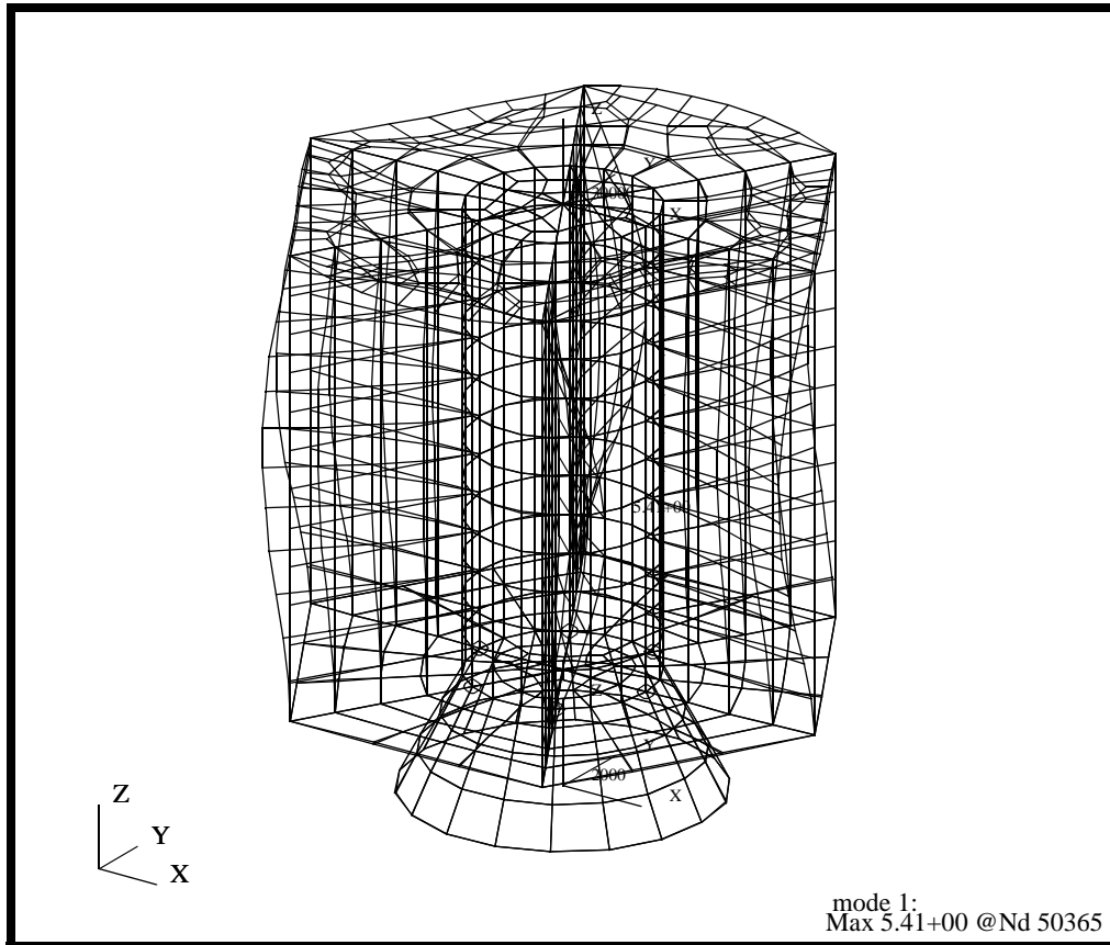
Figure 9.2. Default Eigenvector Deformation Plot
