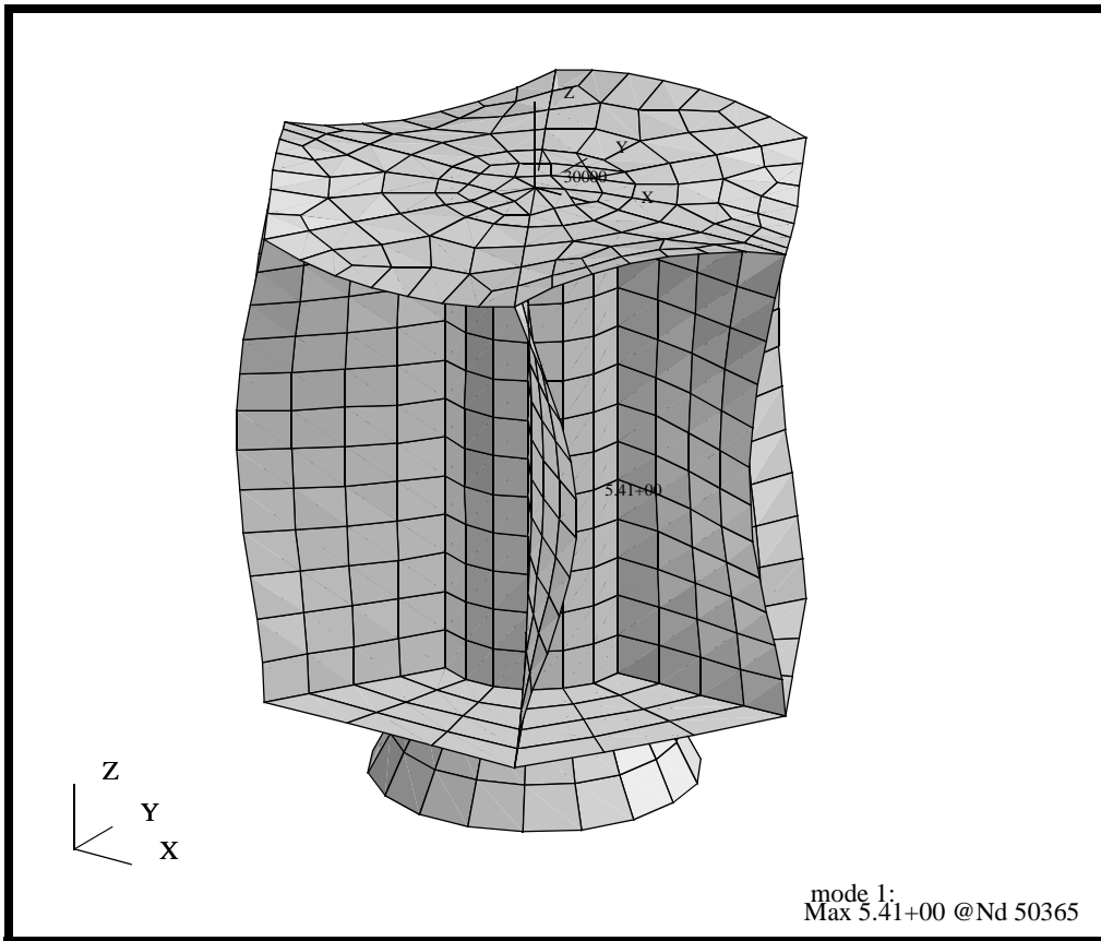
Figure 9.3. Eigenvector Deformation for Mode 1 in Shaded Render style.
