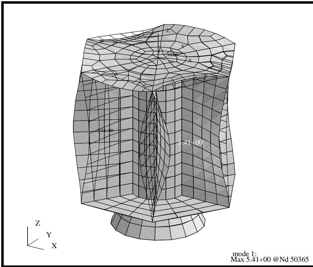
Figure 9.4. Simultaneous Display of the Eigenvector for Modes 1 & 3.
