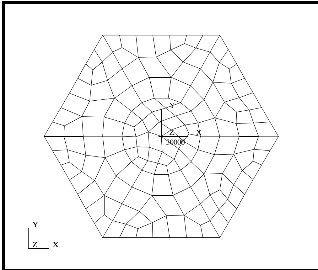
Figure 9.5. Finite elements representing the Upper Platform
