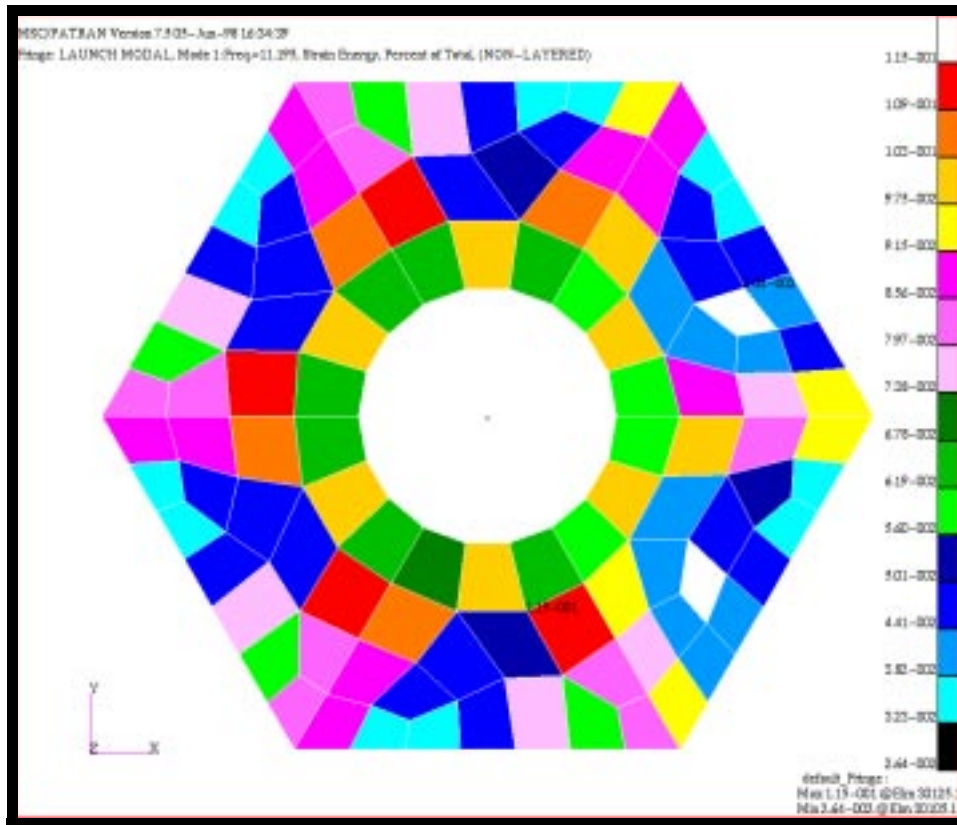
Figure 9.6. Element Strain Energy plot of the Upper Platform.
