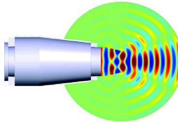
Visualization of the sound directivity generated by an APU exhaust Model courtesy of Airbus
