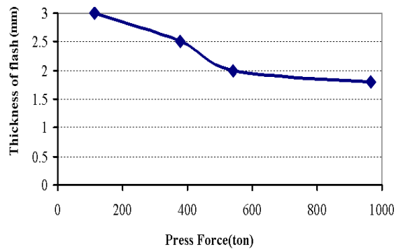
FIGURE 11. Variation of flash thickness with press force
