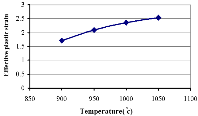
FIGURE 7. Effect of temperature on the maximum effective plastic strain
