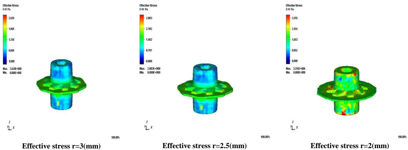
FIGURE 10. The effect of die corner radius on the workpiece stress
