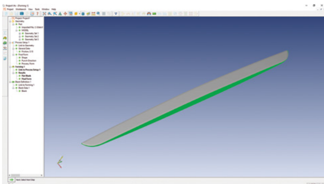
Part and blank development in FormingSuite
