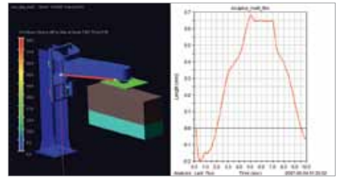
High-speed infeed machine for bottles: ADAMS model
